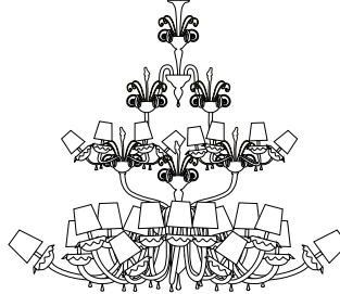
8080/16+8 Ø 185 cm H. 190 cm 125 kg 1,50 mc E 14 led
