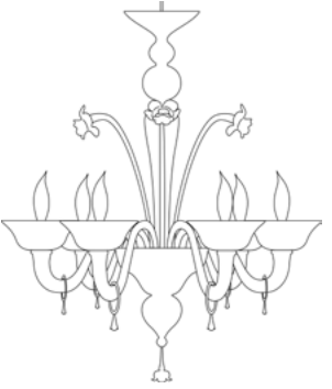
7472/6 Ø 80 cm H. 80 cm 16 kg 0,20 mc E 14 led
