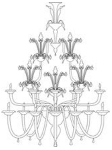
7897/8+8 Ø 180 cm H. 160 cm 80 kg 1,94 mc E 14 led
