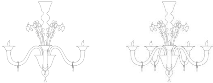
7980/3 Ø 58 cm H. 70 cm 7 kg 0,12 mc E 14 led 7980/5 Ø 75 cm H. 85 cm 12 kg 0,20 mc E 14 led
