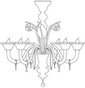
7467/6 Ø 80 cm H. 80 cm 16 kg 0,20 mc E 14 led
